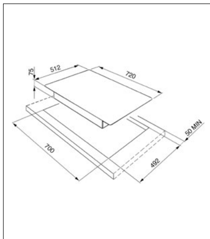
70CM GAS HOB: PGF75-4
