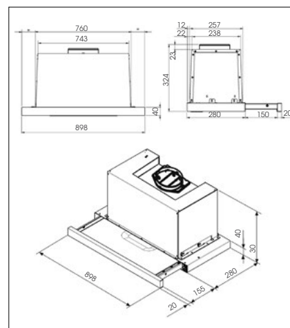
90CM TELESCOPIC EXTRACTOR: KSET900XE
