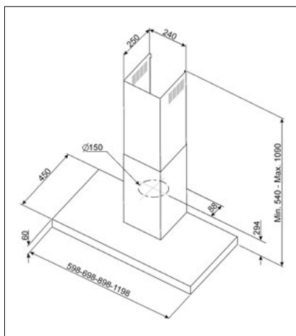
90CM EXTRACTOR: KAT900HX
