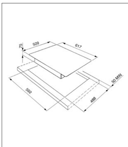
60CM GAS HOB: PGF64-4
