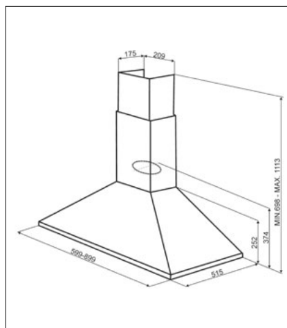
90CM EXTRACTOR: KSA900HX
