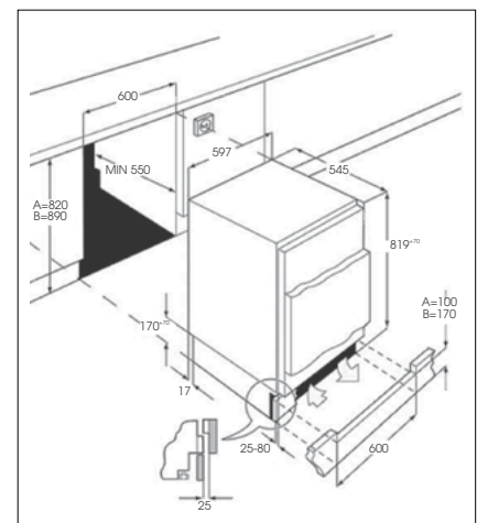
54cm UNDERCOUNTER FRIDGES & FREEZERS: UD7140LSP; UD7108FSEP; UD7122CSP
