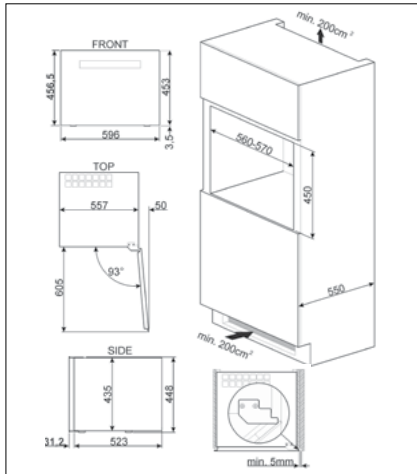
60x45cm COMPACT WINE COOLER: CVI318X
