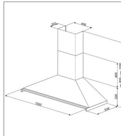
150CM EXTRACTOR: KD150XE
