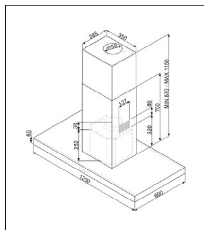
120CM EXTRACTOR: KI120XE
