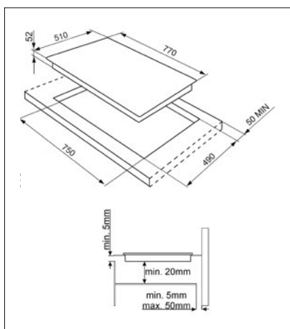
77CM INDUCTION HOB: SIM581B
