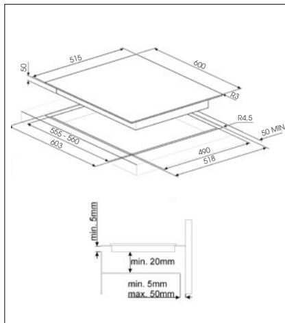
60CM INDUCTION HOB: SI5641D
