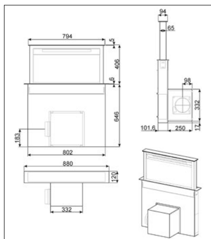
90CM DOWNDRAFT EXTRACTOR: KDD90VXE-2
