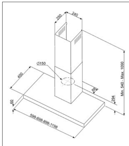
60CM EXTRACTOR: KAT600HX
