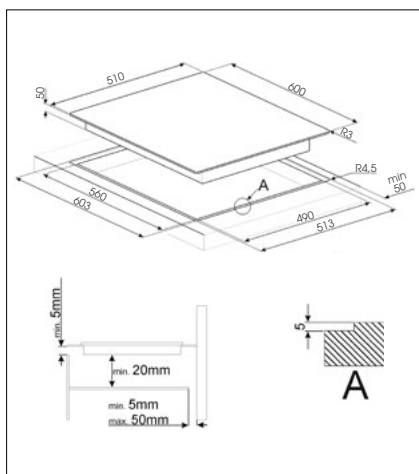
60CM INDUCTION HOB: SIM662DW
