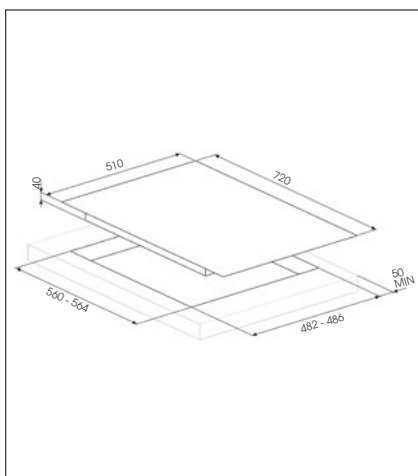
72CM GAS-ON-GLASS HOBBS: PV175CB; PV175S-1/B-1/N-1
