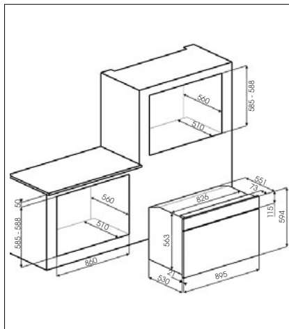
90CM SINGLE OVEN: SF9300GGVX1
