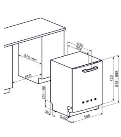
60CM DISHWASHER: ST2FAB
