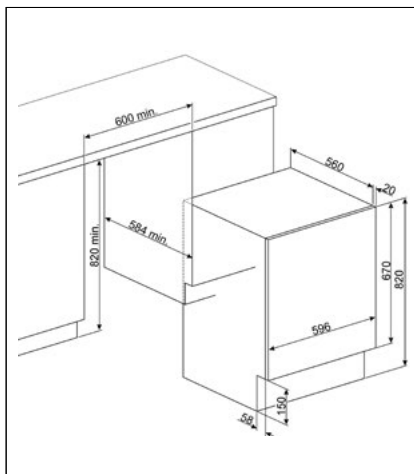
60CM WASHING MACHINE & WASHER DRYER: LST127-2; LSTA147S
