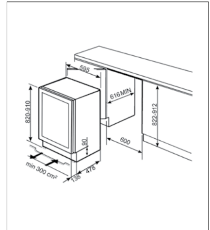
82cm UNDERCOUNTER WINE COOLER: CVI338X
