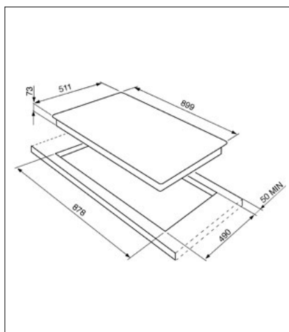
90CM GAS HOB: PS906-4
