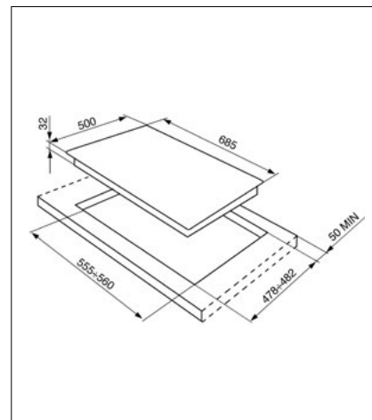
70CM GAS HOB: SR975PGH/XGH/NGH
