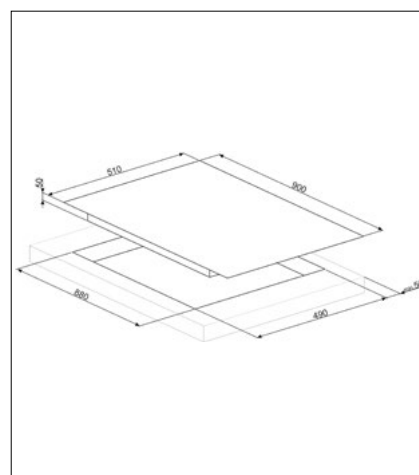
90CM INDUCTION HOB: SIM693DW
