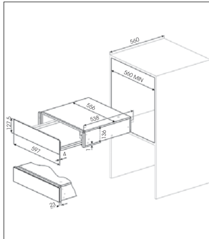
15cm SOMMELIER DRAWER: CTPS313X
