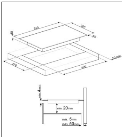
30CM CERAMIC HOB: SE332EB
