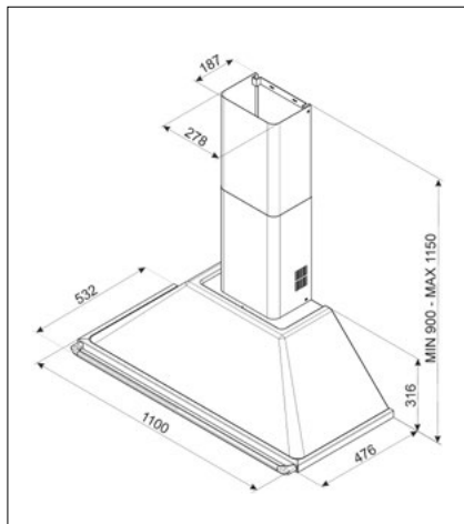
110CM EXTRACTORS: KT110PE/XE/BLE
