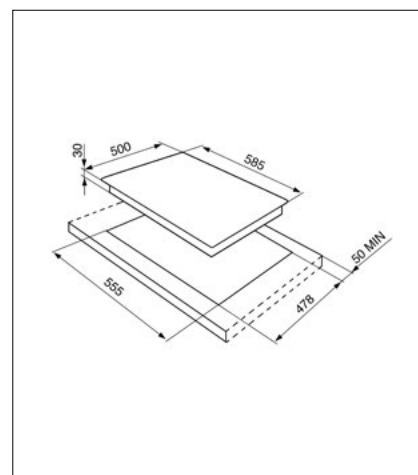
60CM GAS HOB: PS60GHC
