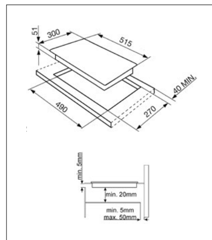
30CM INDUCTION HOB: SI5322B
