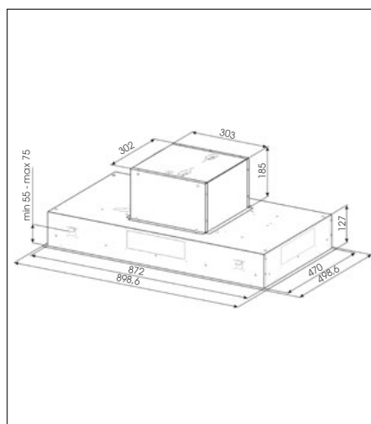
90CM CEILING EXTRACTOR: KSEG90XE-2
