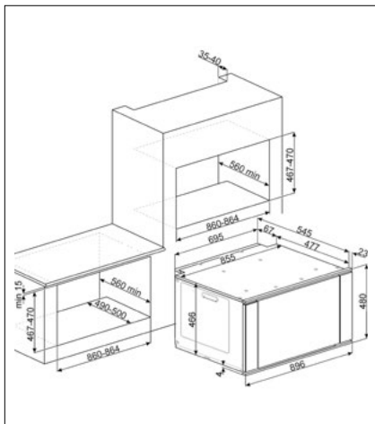
90CM SINGLE OVEN: SF9310XR
