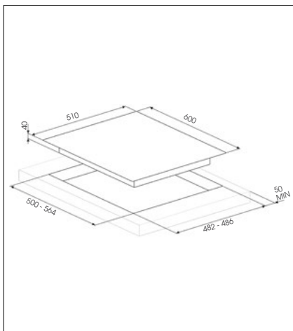
60CM GAS-ON-GLASS HOBS: PV164S-1/B-1/N-1
