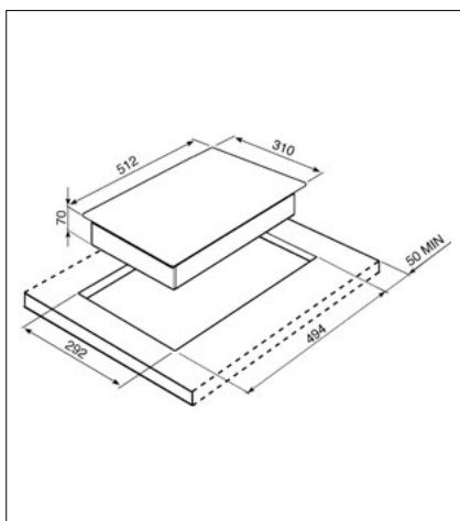
30CM ASSORTED HOBBS: PGF30T-1; PGF32I-1; PGF30B; PGF32C; PGF32G; PGF31G-1
