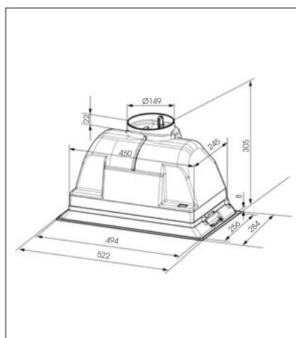
70CM FULLY INTEGRATED EXTRACTOR: KSEG5XE
