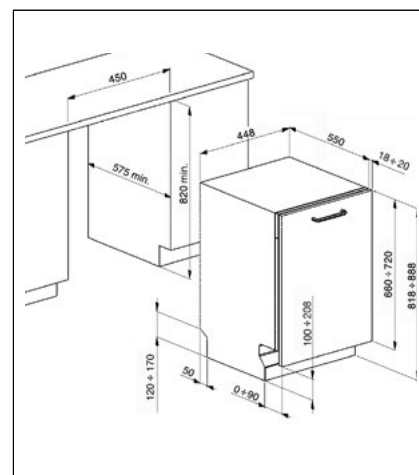
60CM DISHWASHER: DWI4SSA
