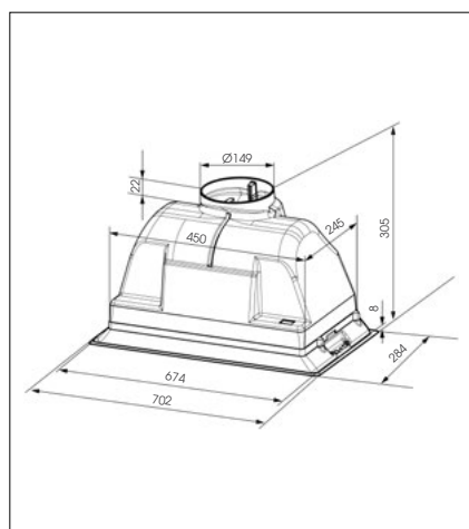
70CM FULLY INTEGRATED EXTRACTOR: KSEG7XE
