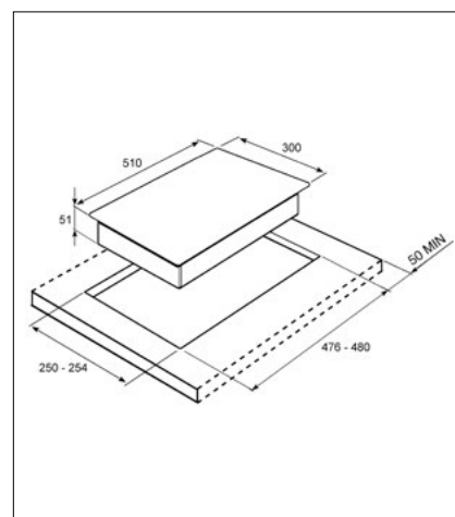
30CM GAS-ON-GLASS HOB: PC32GNO; PC31GNO
