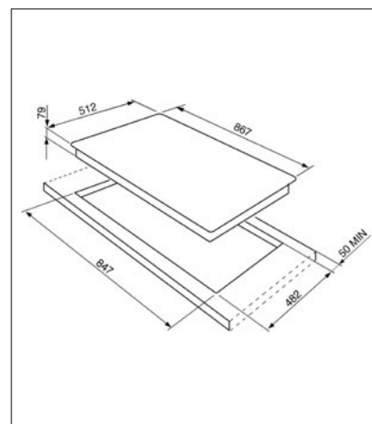
90CM GAS HOB: PGF95-4
