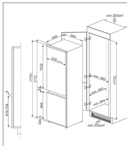
54cm FRIDGE-FREEZERS: C3172NP; C3170P
