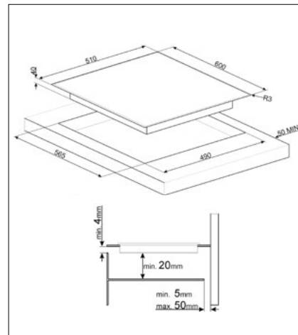
60CM CERAMIC HOB: SE364TD
